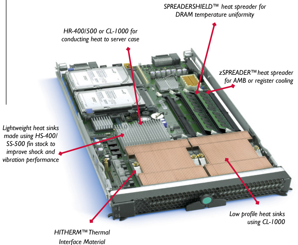
HITHERM™ Thermal Interface Material
